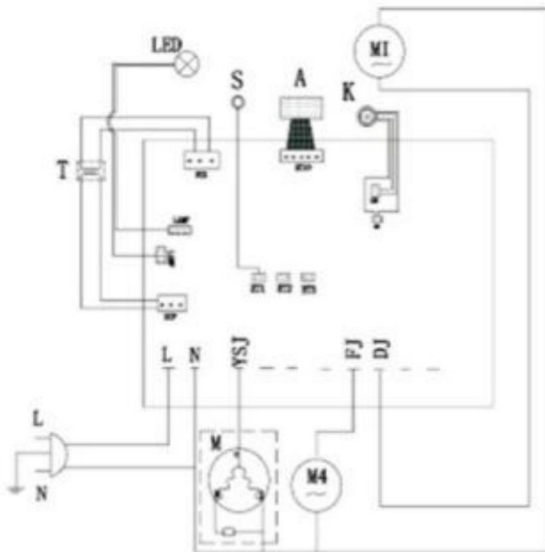
Electrical diagram-XRJ4LX1
