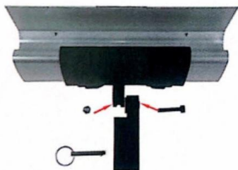
3. Fix screw assembly.
