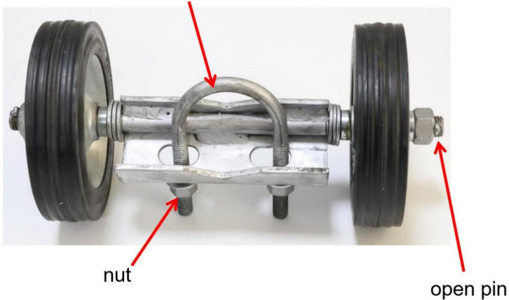
U-shaped bolt
