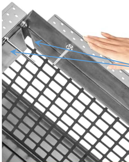
Inner reinforced edge strip A/B
