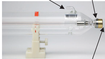
Water Outlet(Upturn) Negative Electrode(-)
