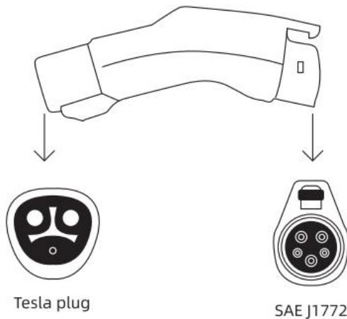
SAE J1772
