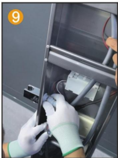
9 Connect the water outlet connector and hand spray seat joint
