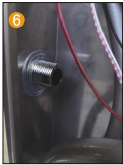
6 Insert the hand spray nozzle into the panel and install the gasket
