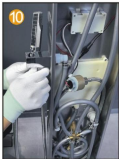
10 Connect the hand spray hose to the handheld shower head
