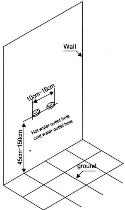
Reserved water layout
