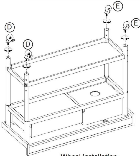
Wheel installation
