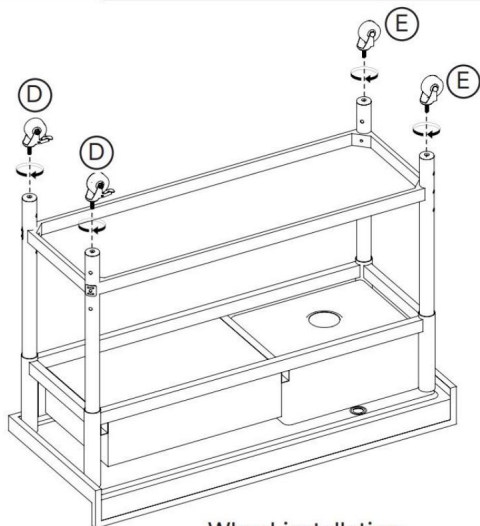
Wheel installation
