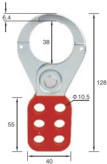
PA COATED STEEL HASP - RING BD-K02
