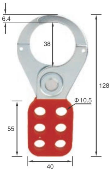
PA COATED STEEL HASP- R0-K02
