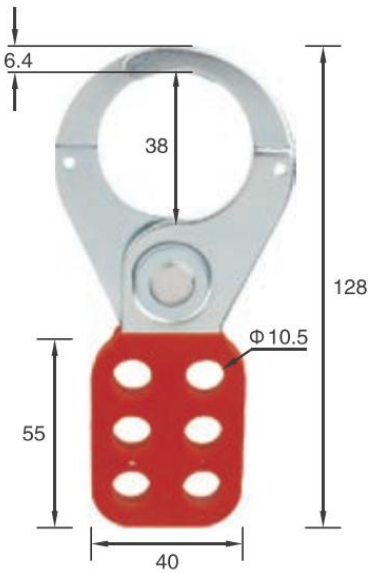
PA COATED STEEL HASP · BD-K02
