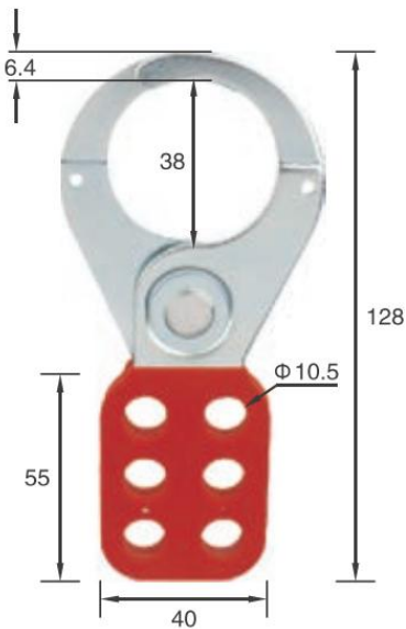
PA COATED STEEL HASP · RING
