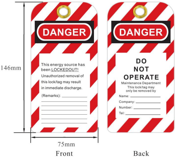
BD-P01 Thickness : 0.45mm Material : PVC
