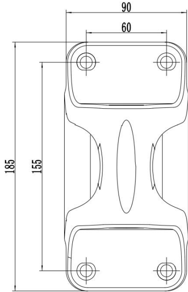
Hole for Plastic Wall Bracket
